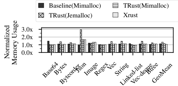
Figure 11: Normalized memory usage of TRUST and XRust tested with the 11 widely used crates.
